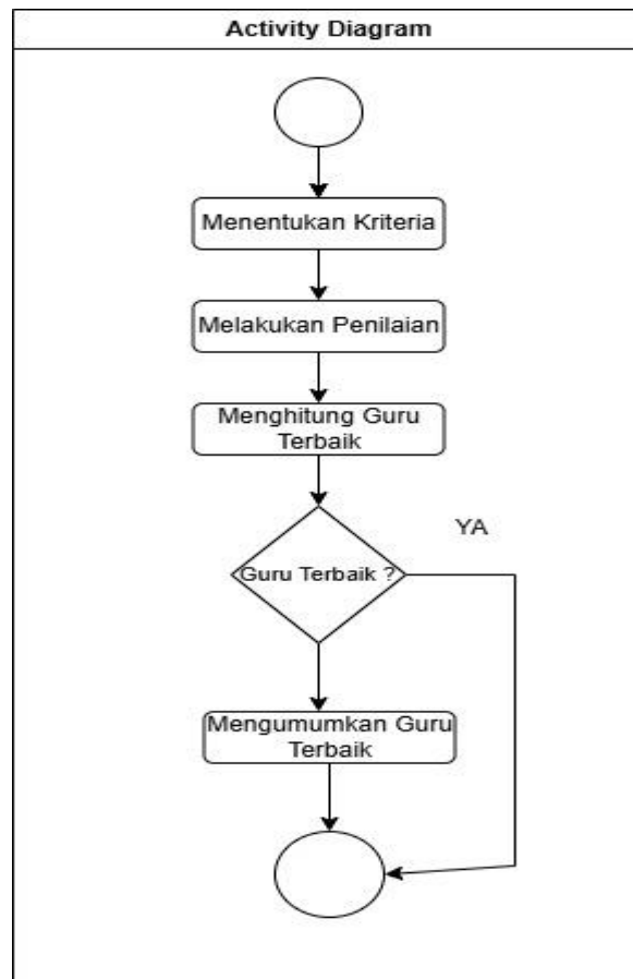
Gambar 3. 1 Activity Diagram
